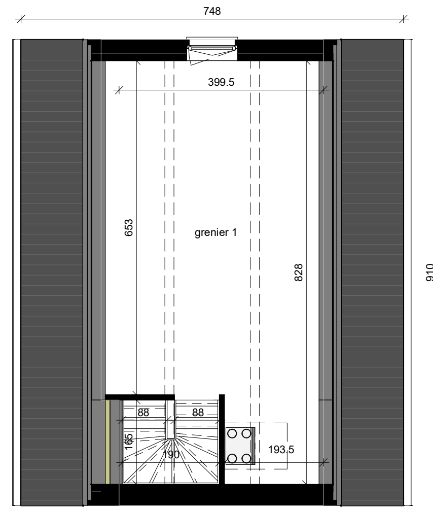
grenier surf. brute 38.85 m²
